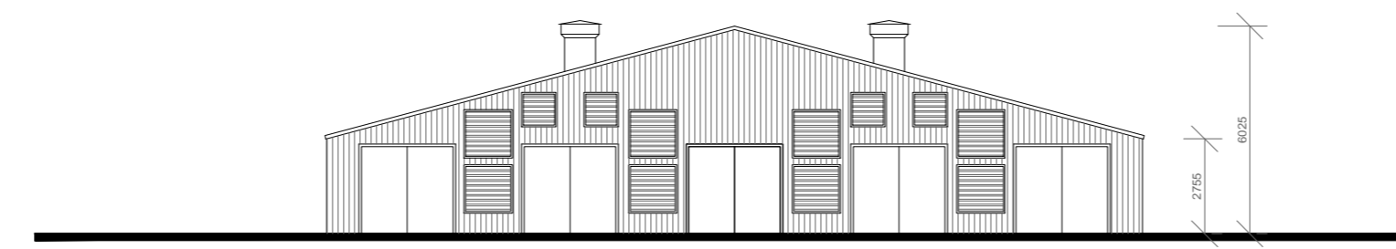
North West (End) Elevation 1:200
