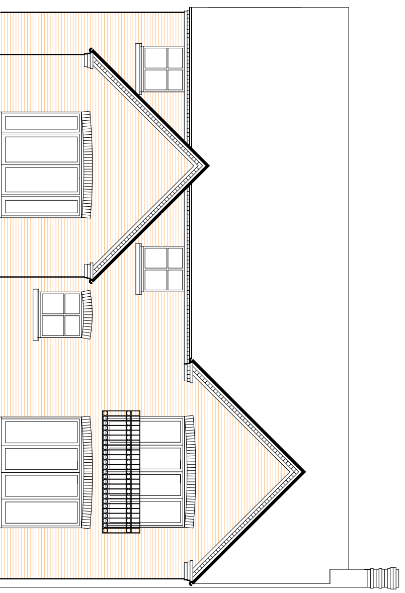
front elevation south west
