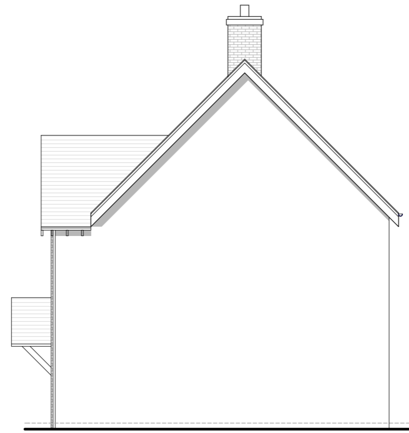
SIDE ELEVATION
