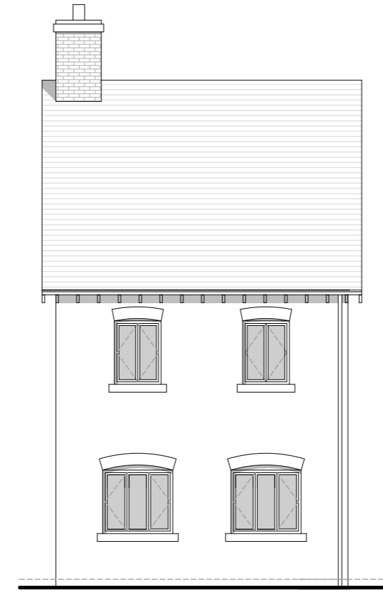
REAR ELEVATION
