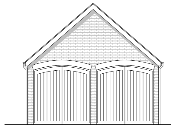
FRONT ELEVATION
