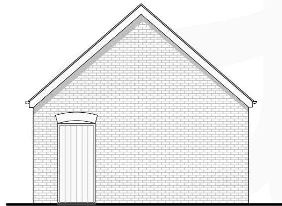
REAR ELEVATION
