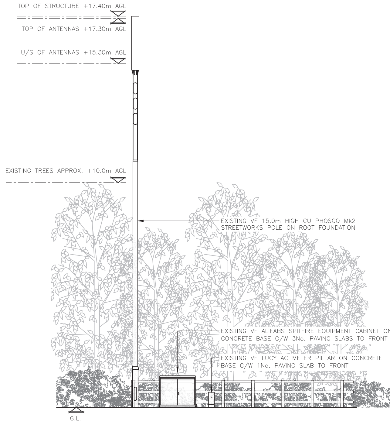
EXISTING SOUTH ELEVATION (1:100)
