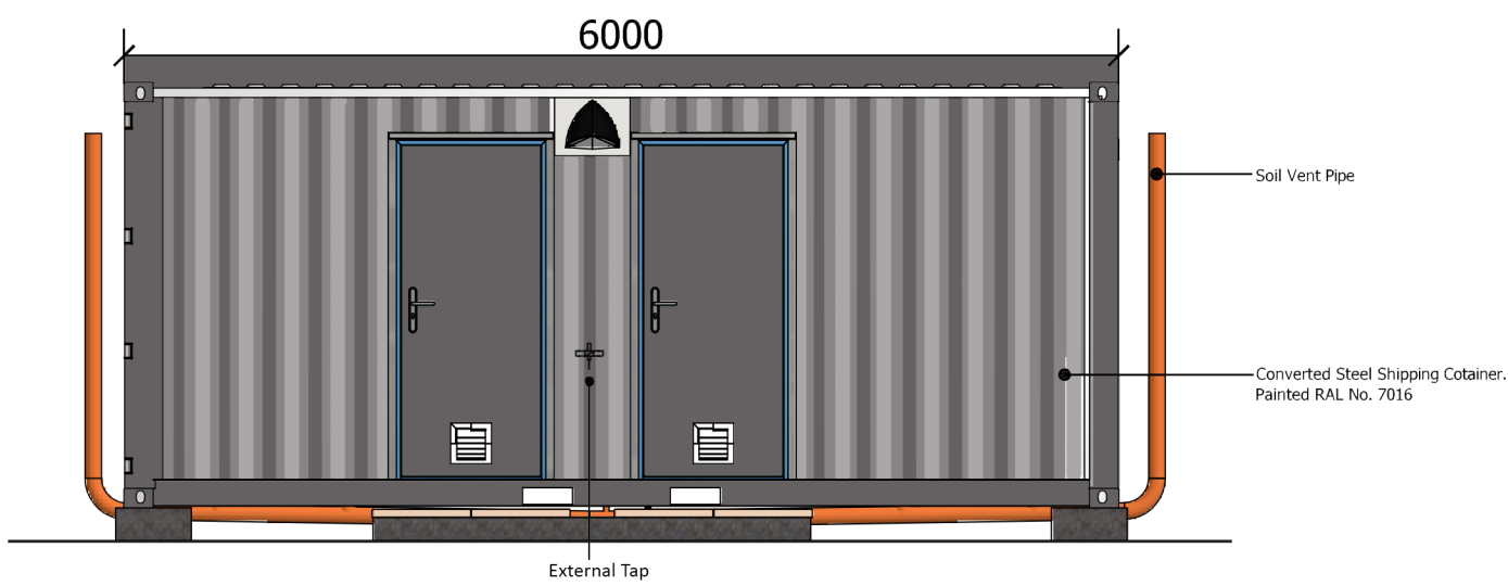
Proposed Elevation 1
