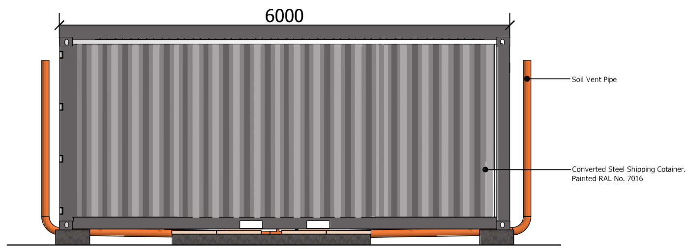
Proposed Elevation 3
