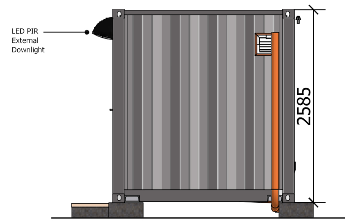
Proposed Elevation 4
