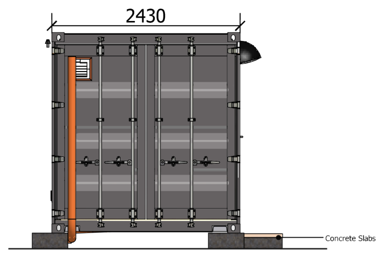
Proposed Elevation 2
