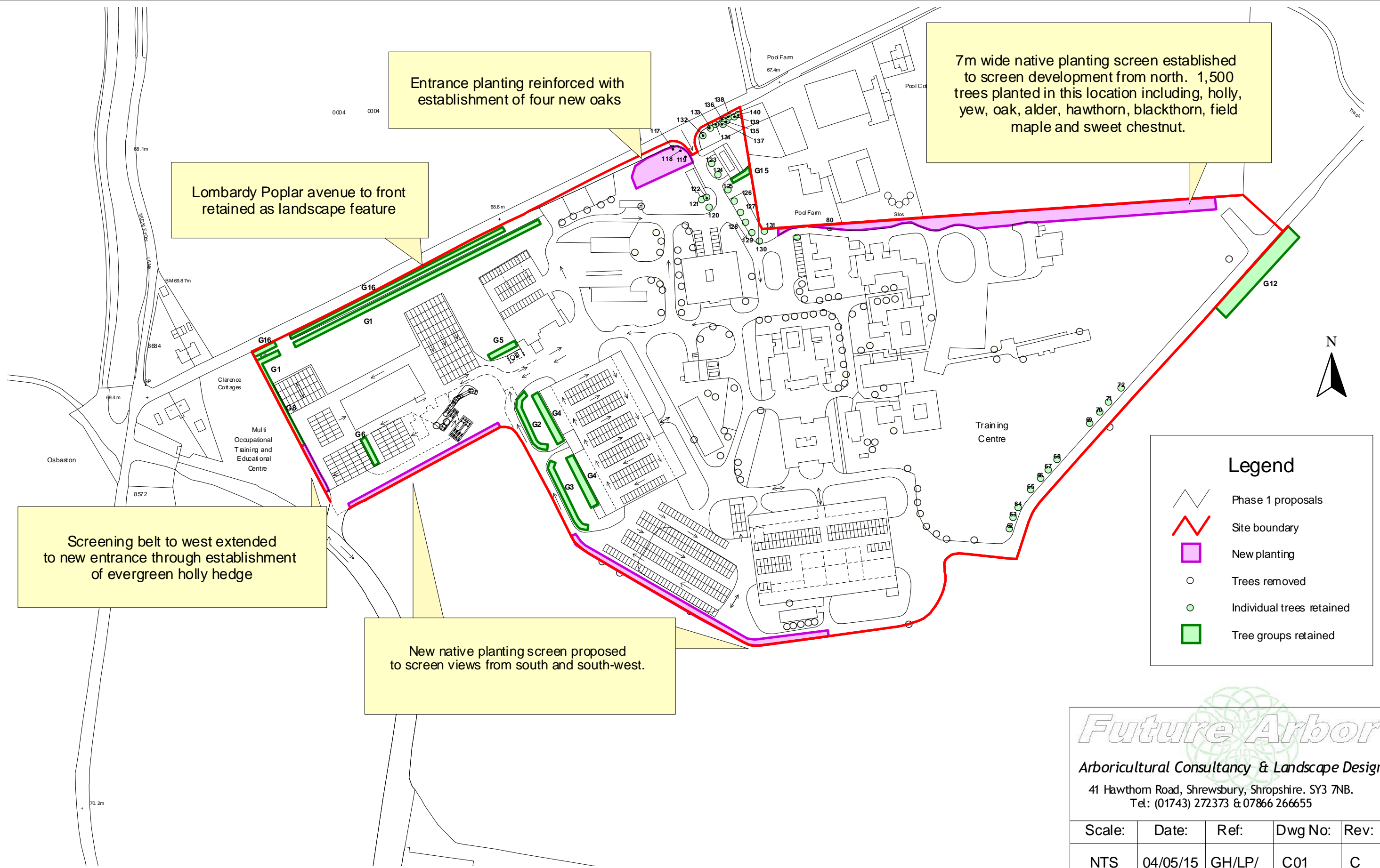
Plan 7c: Proposed final landscaping plan superimposed over parking proposals (Phase 1) at The Angel Centre, High Ercall, TF6 6RB. Plan shows additional native planting to screen views from south and south-west.
