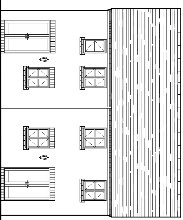
REAR ELEVATION
