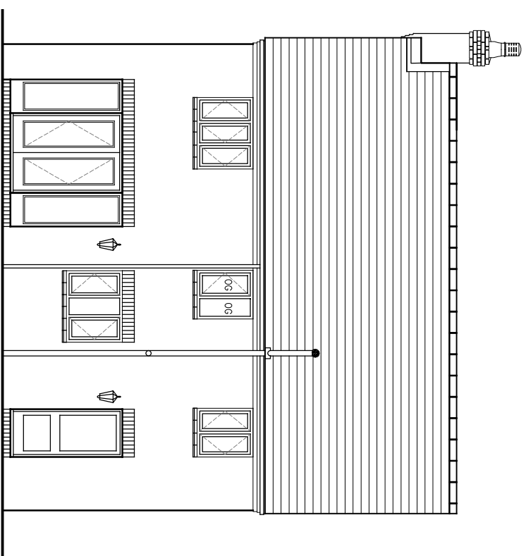
REAR ELEVATION
