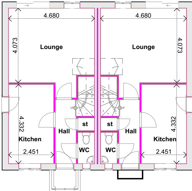
PLOTS 3, 4, 7, 8 Ground Floor Plan
