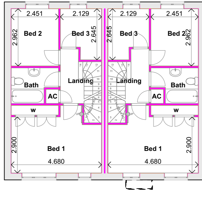
PLOTS 3, 4, 7, 8 First Floor Plan
