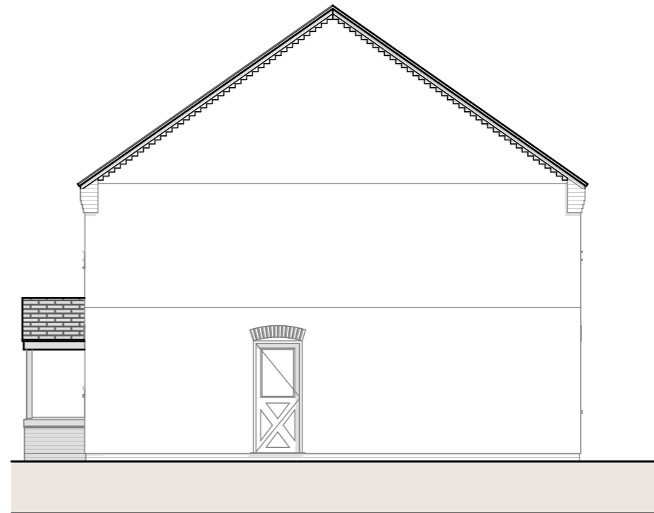
5, 6, 9, 10, 15-17 RIGHT ELEVATION 1:100
