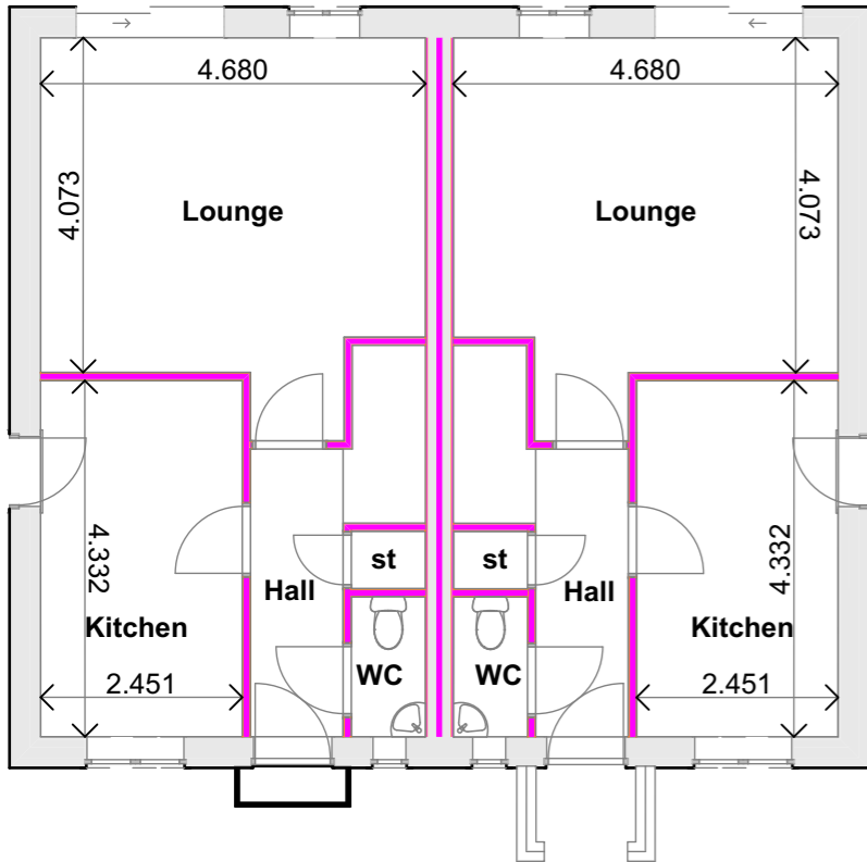
5, 6, 9, 10, 15-17 Ground Floor Plan 1:100
