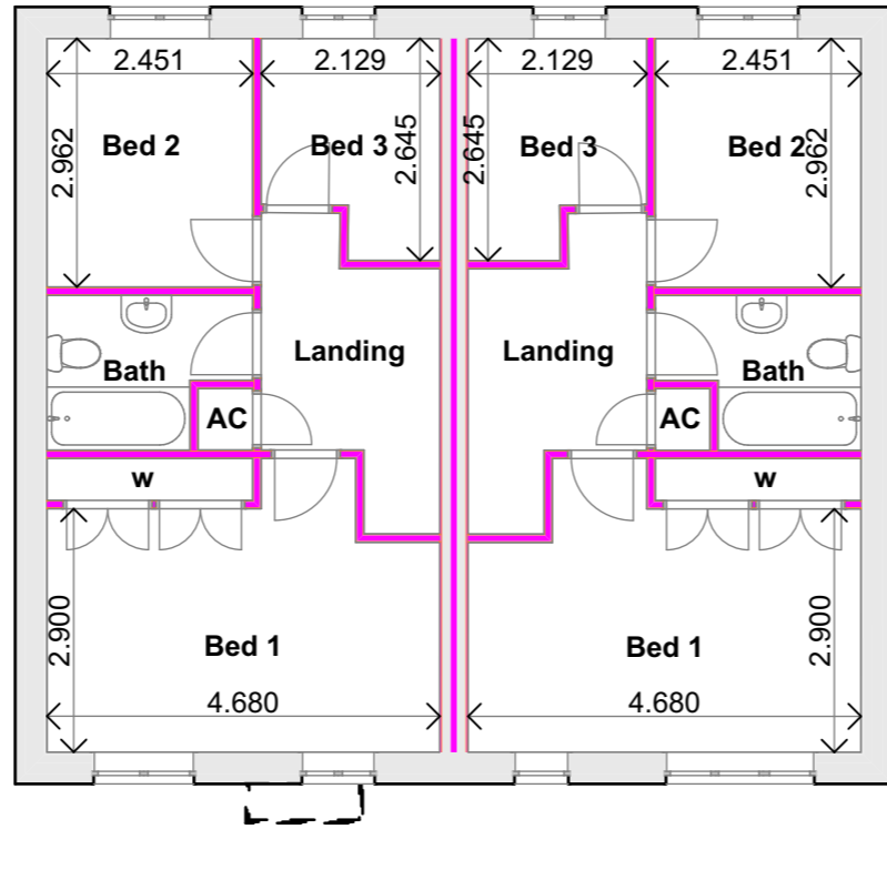
5, 6, 9, 10, 15-17 1ST Floor Plan
