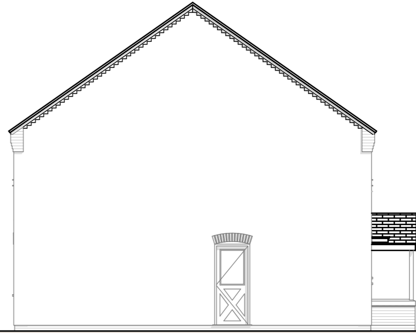
5, 6, 9, 10, 15-17 LEFT ELEVATION
