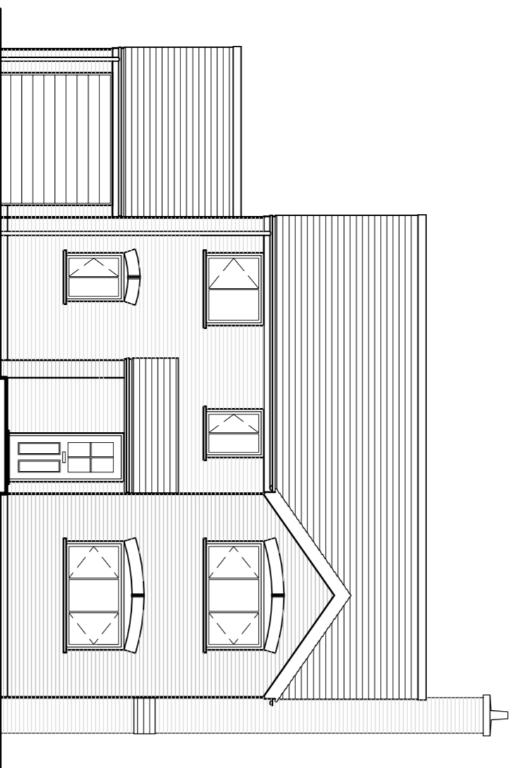
Front Elevation
