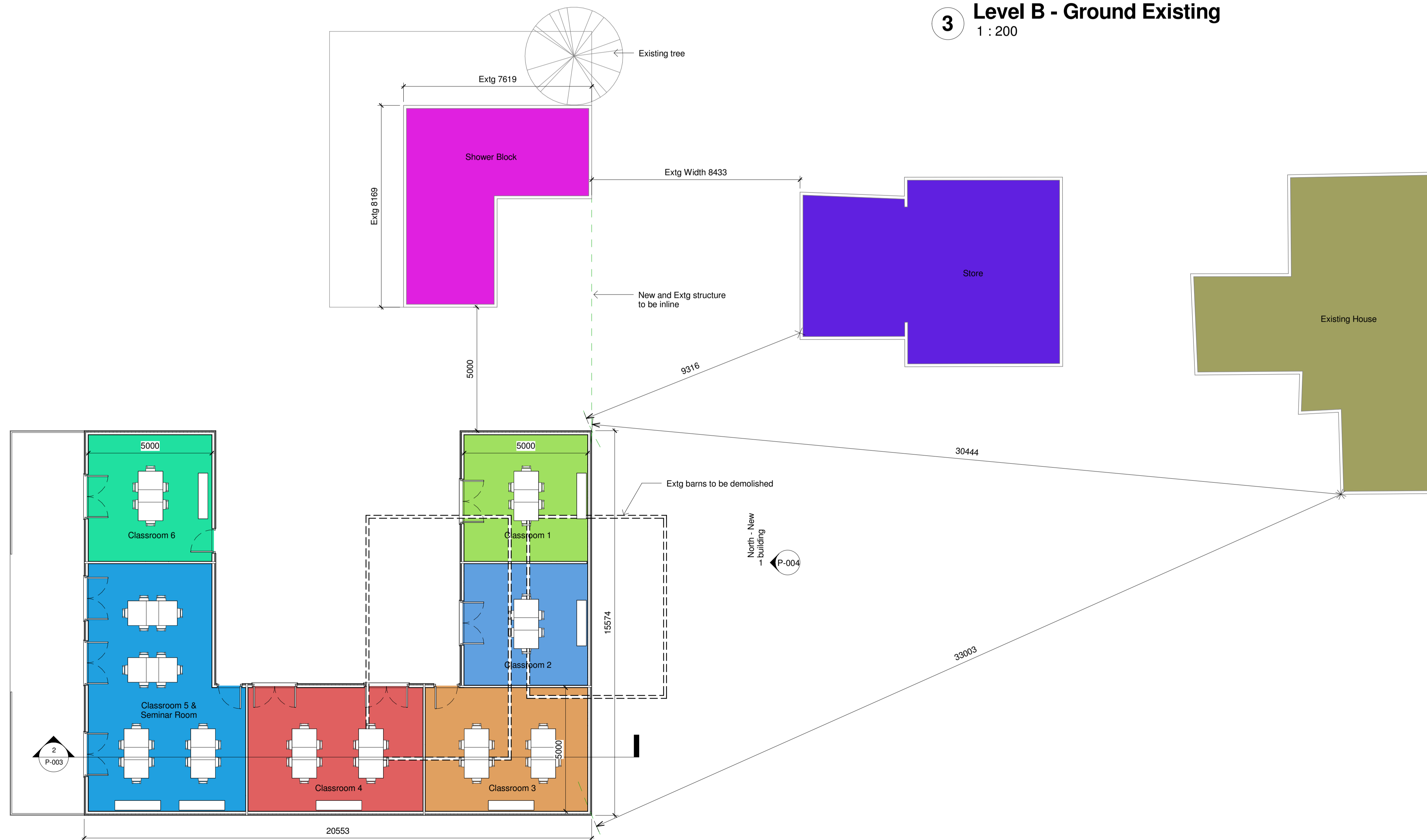
1 Level B - Ground Proposed 1 : 100
