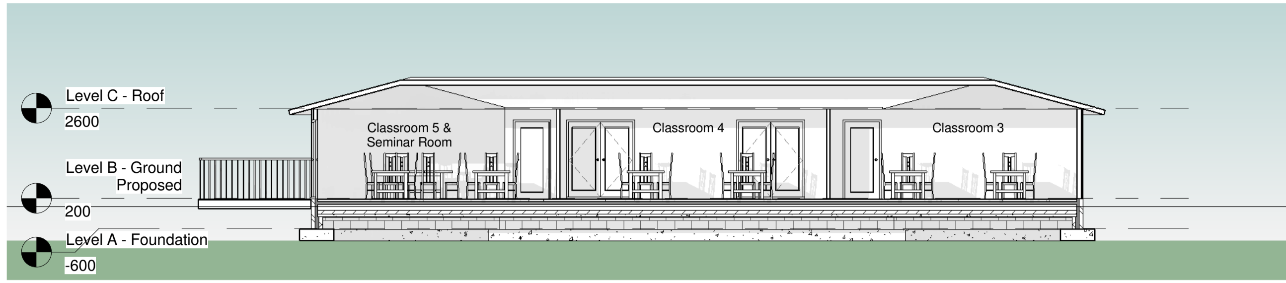
2 Typical Section thro New building 1 : 100
