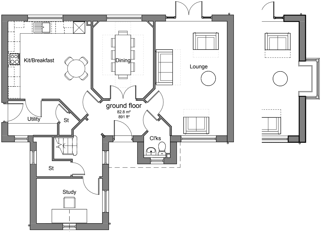
ellesworth traditional render ellesworth cottage render ground floor 1 : 100
