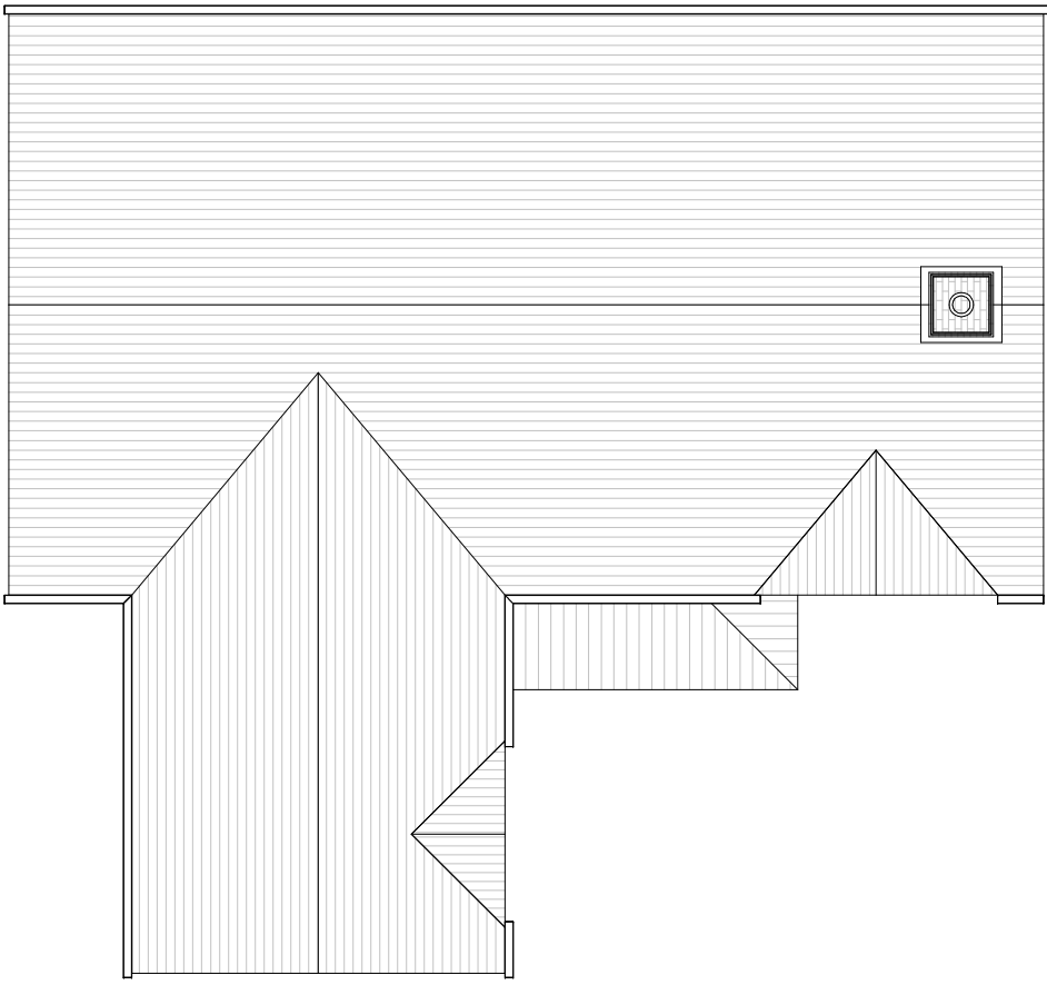
ellesworth traditional roof plan 1 : 100
