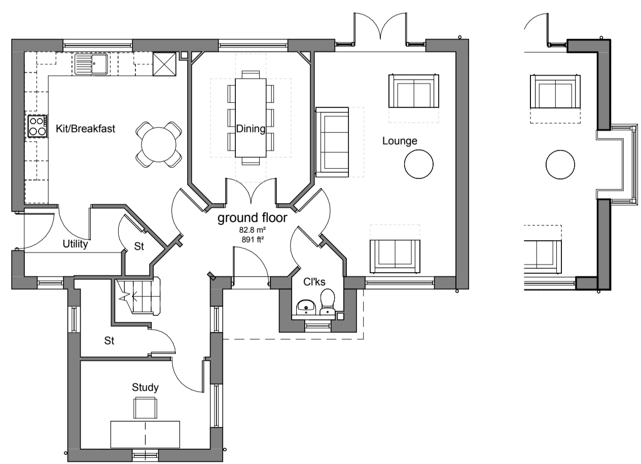
ellesworth traditional render ellesworth cottage render ground floor 1 : 100
