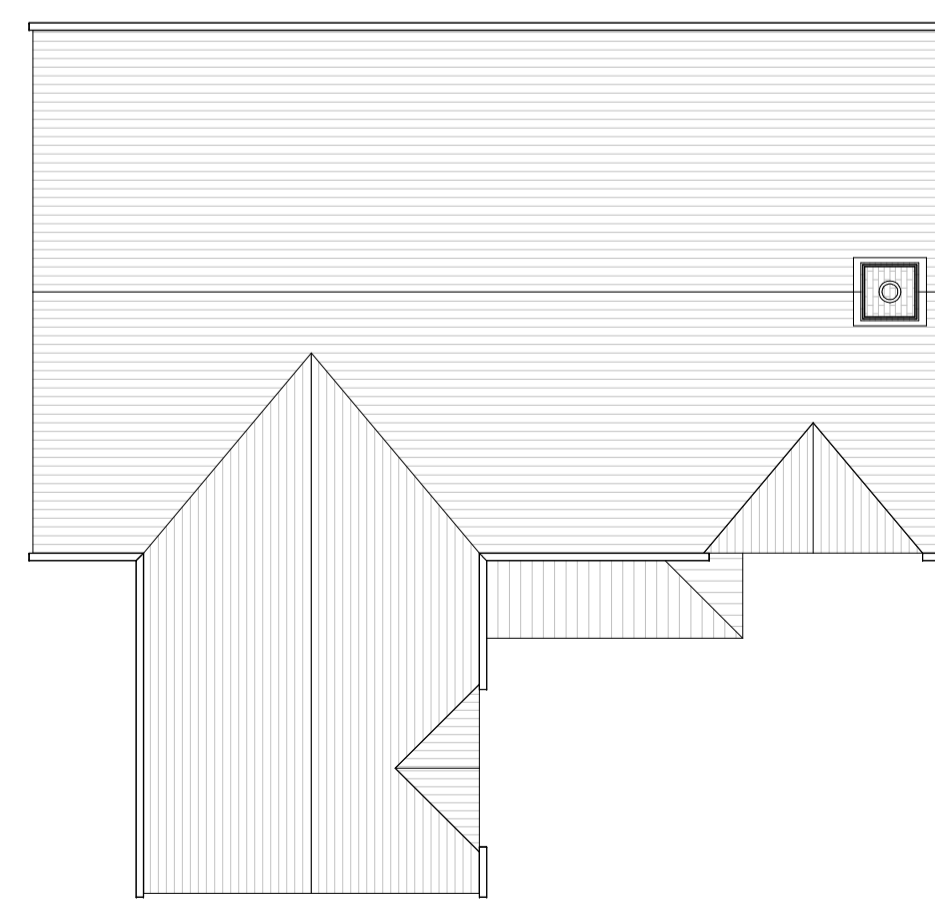
ellesworth traditional roof plan 1 : 100
