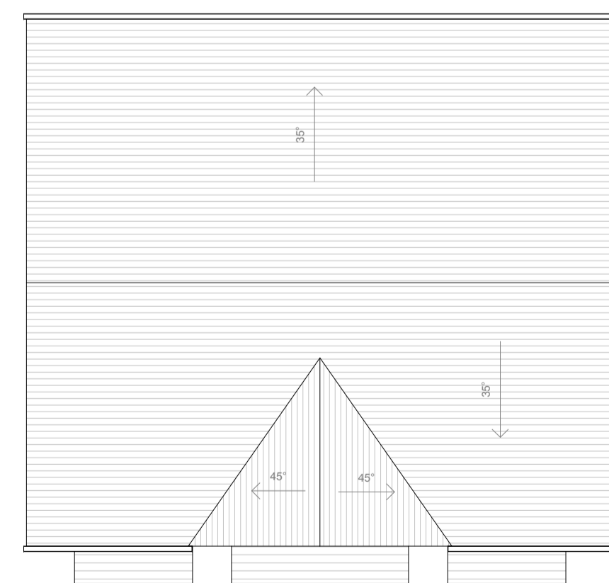
holmewood traditional boarded roof plan 1 : 100
