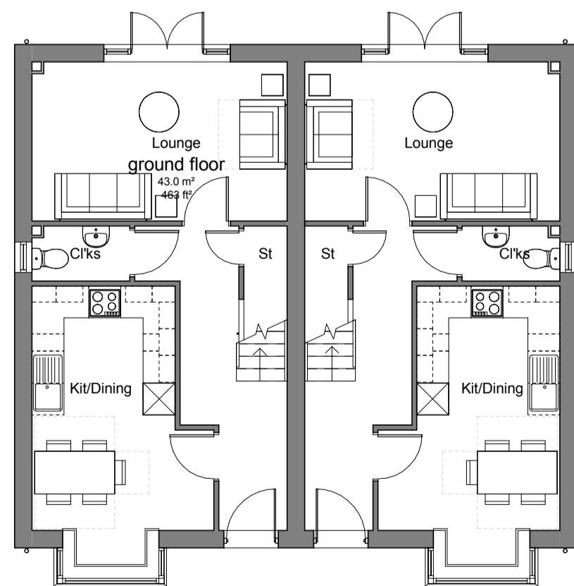
holmewood traditional boarded ground floor 1 : 100
