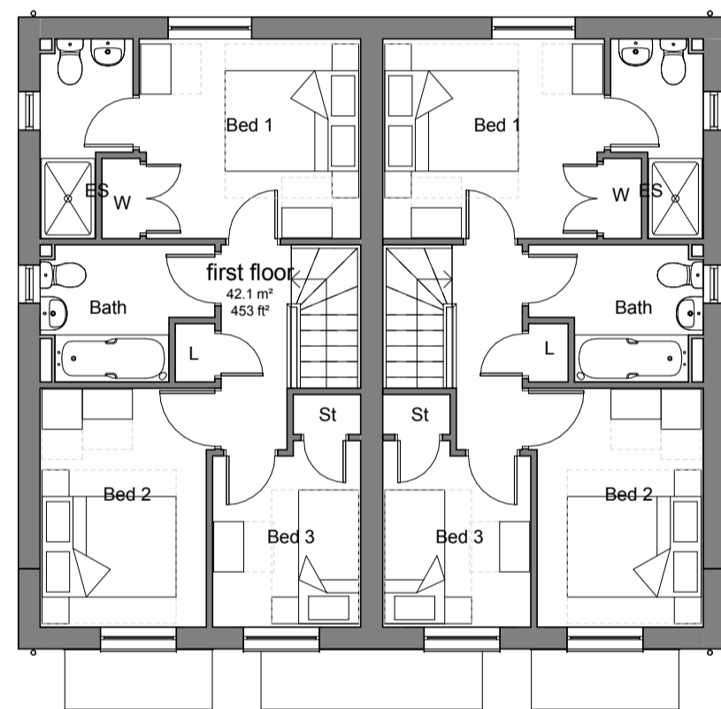
holmewood traditional boarded first floor 1 : 100
