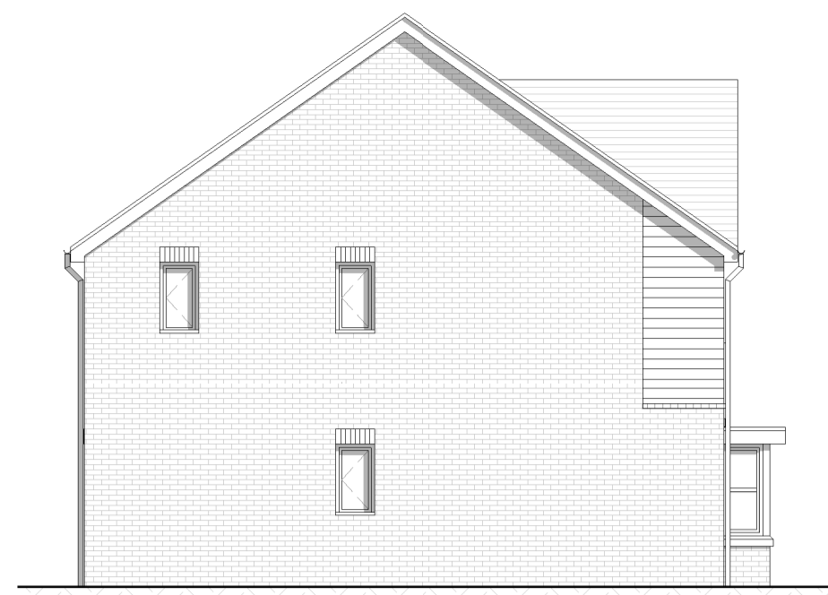
holmewood traditional boarded left elevation 1 : 100
