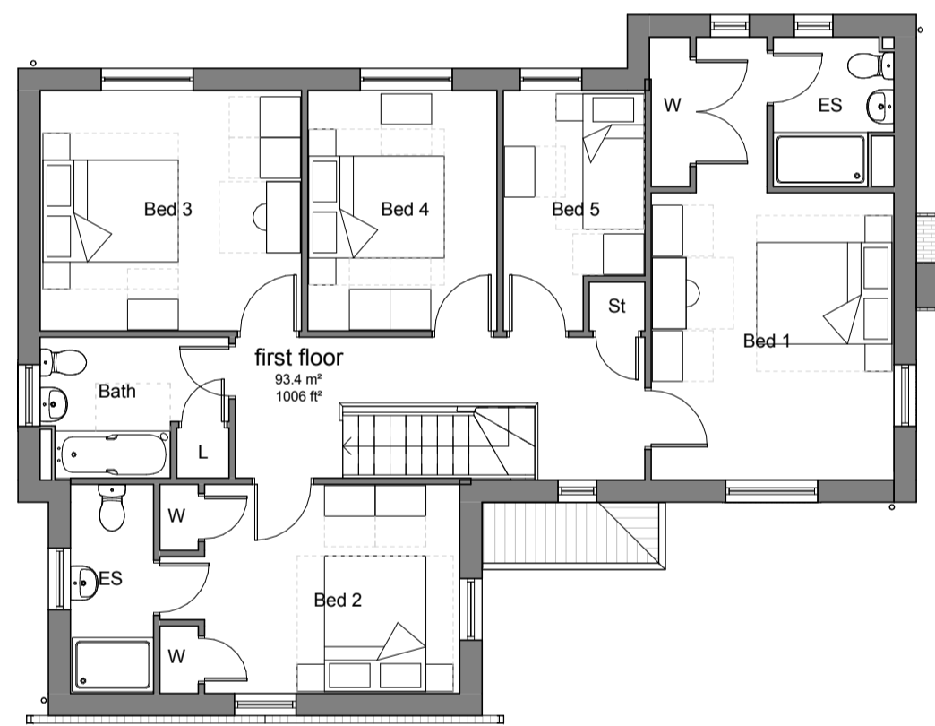
ludworth CT cottage render first floor 1 : 100
