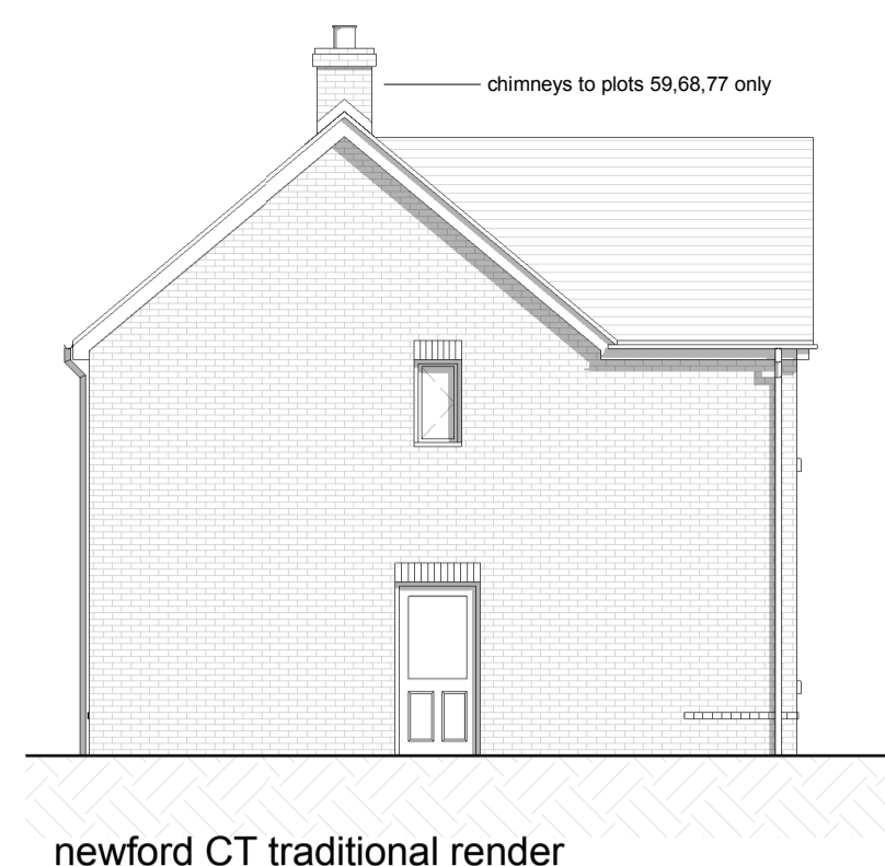
newford CT traditional render left elevation 1: 100
