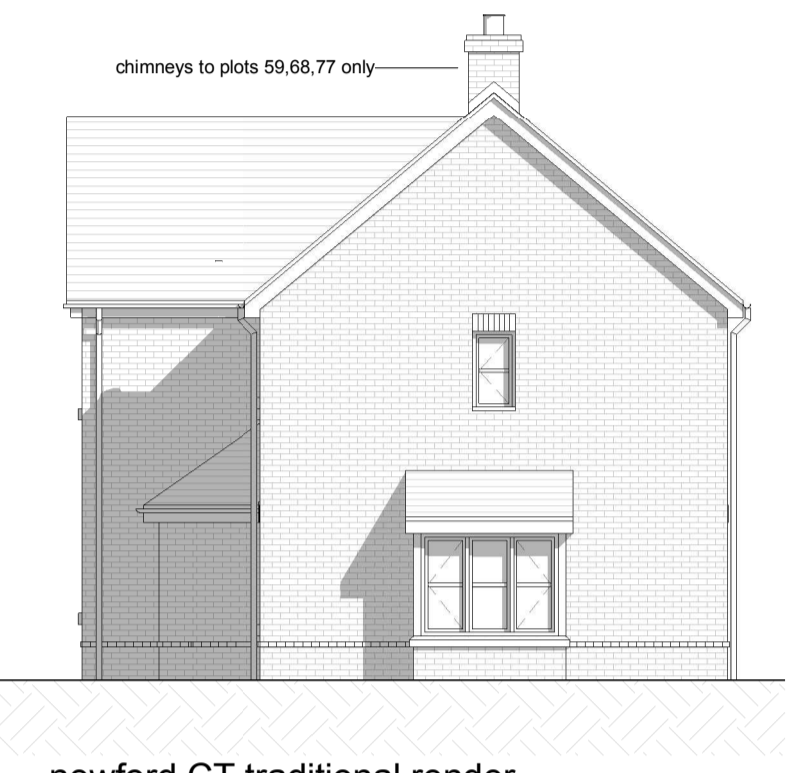
newford CT traditional render right elevation 1: 100
