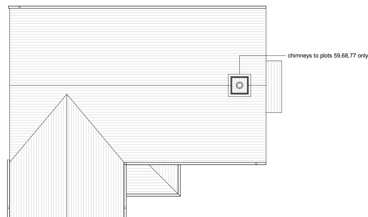
newford CT traditional render roof plan 1: 100
