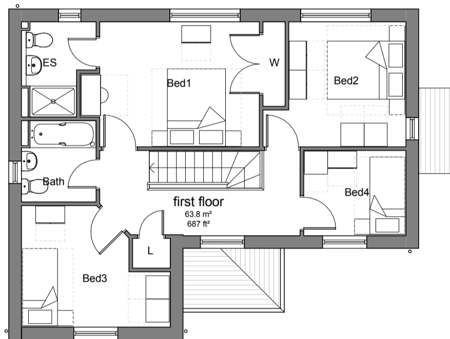
newford CT cottage render newford CT traditional render first floor 1: 100
