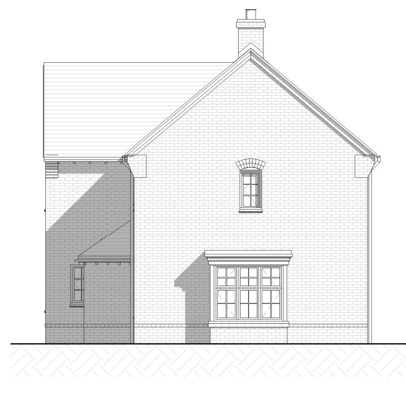
newford CT cottage render right elevation 1: 100
