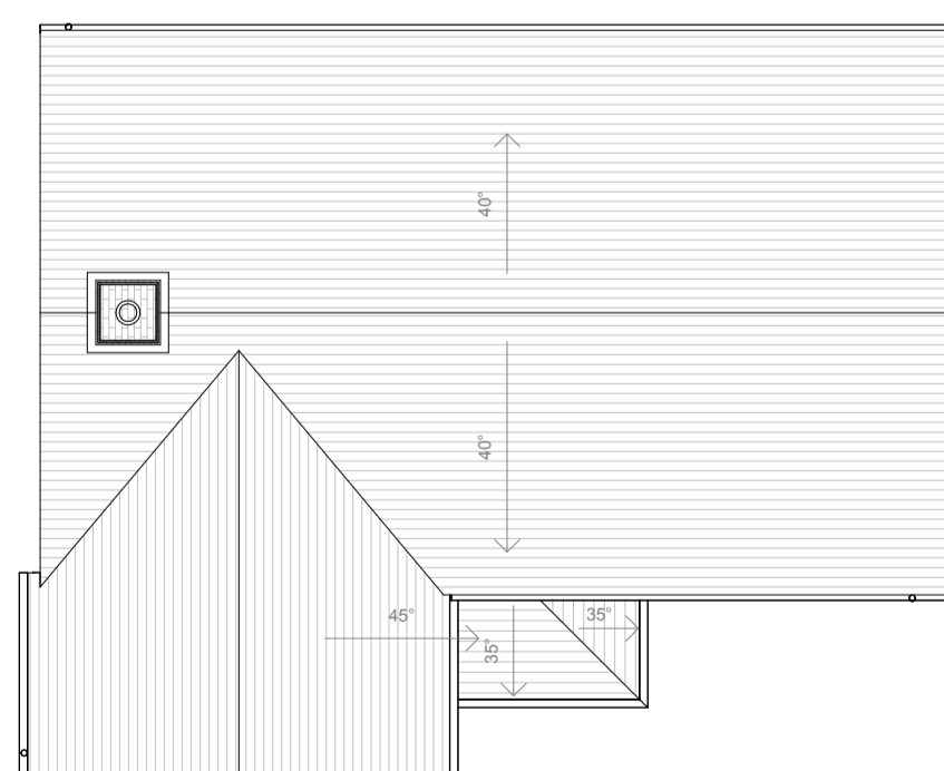
newford CT cottage render roof plan 1: 100
