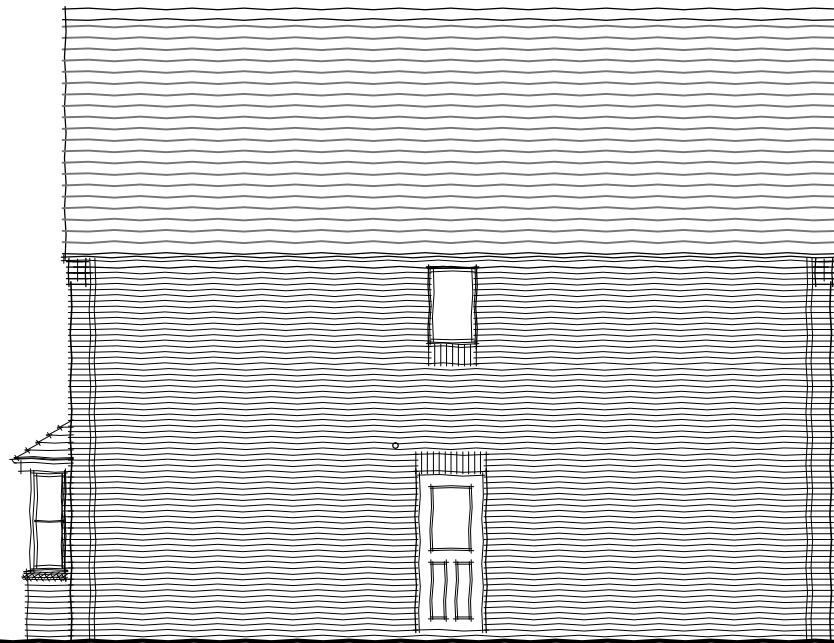
Rear Elevation
