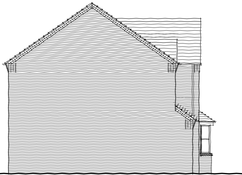
Side Elevation 1
