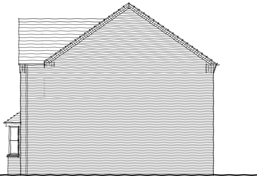
Side Elevation 2
