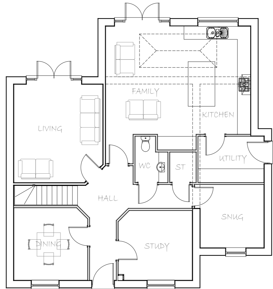
GROUND FLOOR PLAN Plots 11 & 13
