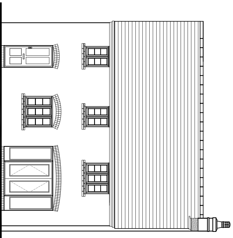
REAR ELEVATION
