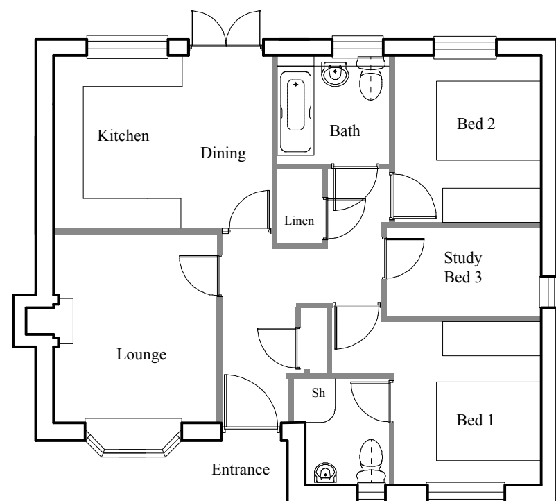
PLAN LAYOUT
