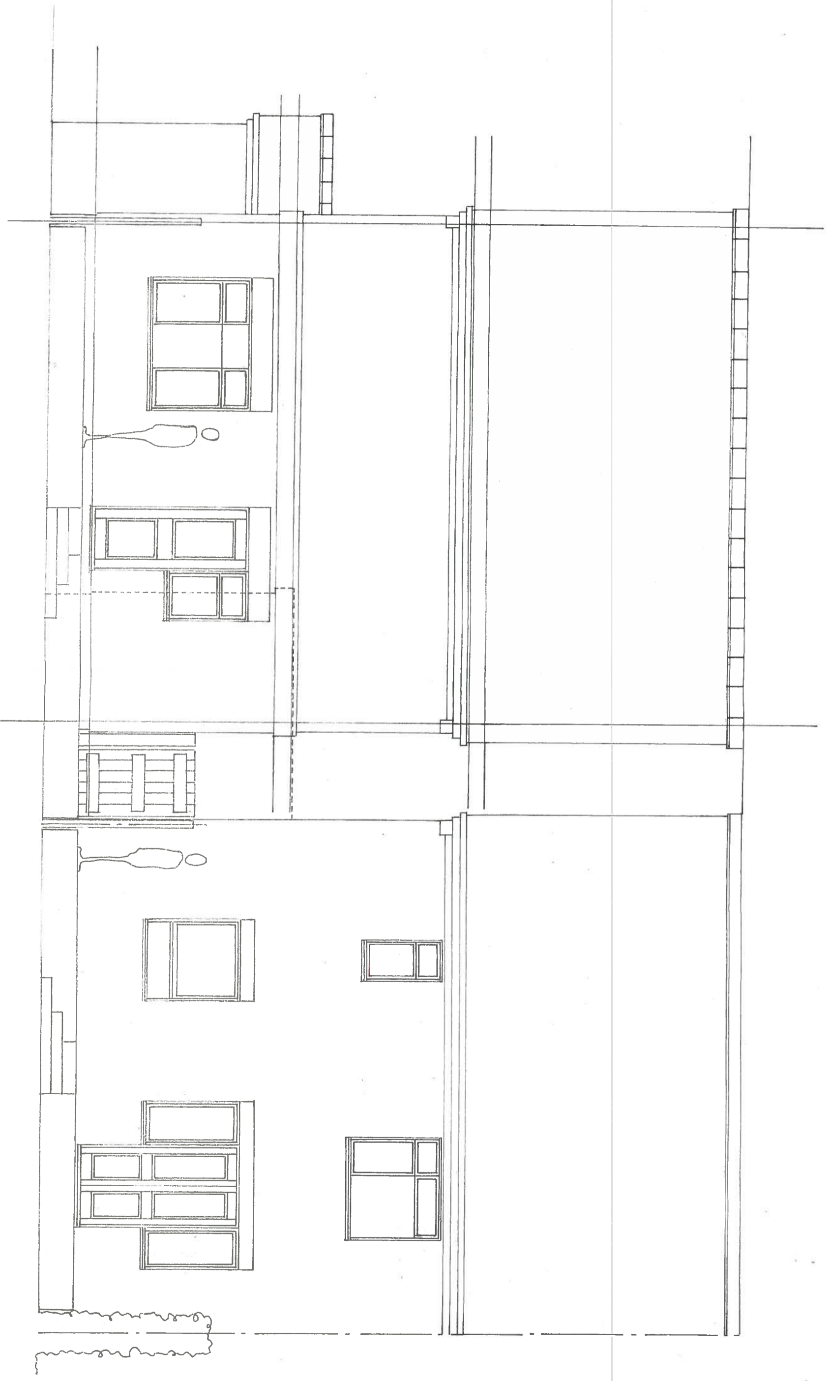
Proposed East Elevation – 1:50
