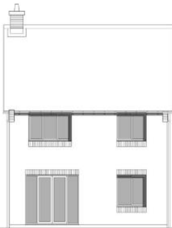
Rear Elevation
