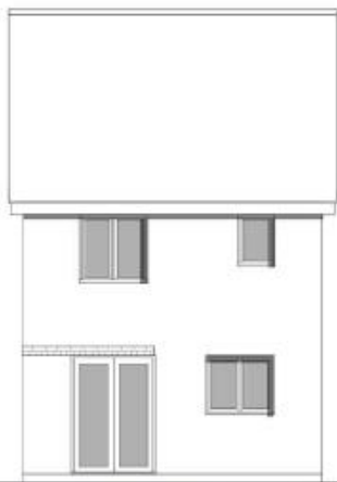
Rear Elevation
