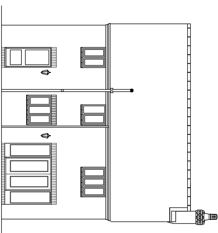
REAR ELEVATION
