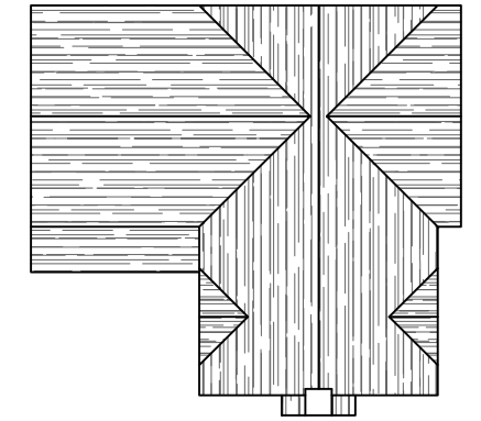
Roof Plan 1/200
