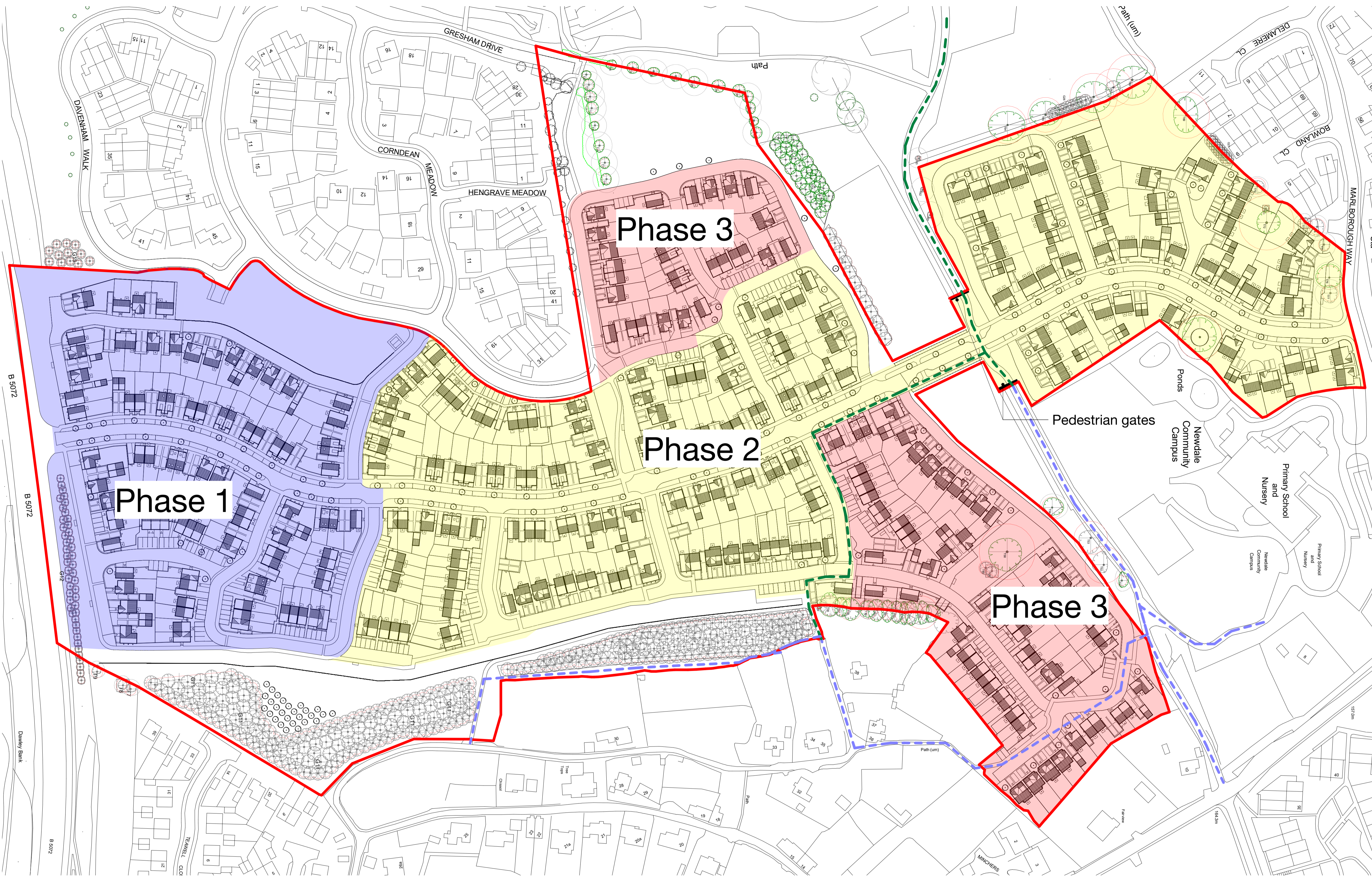
Site - Diagram - Temporary footpath - construction 1 : 1000
