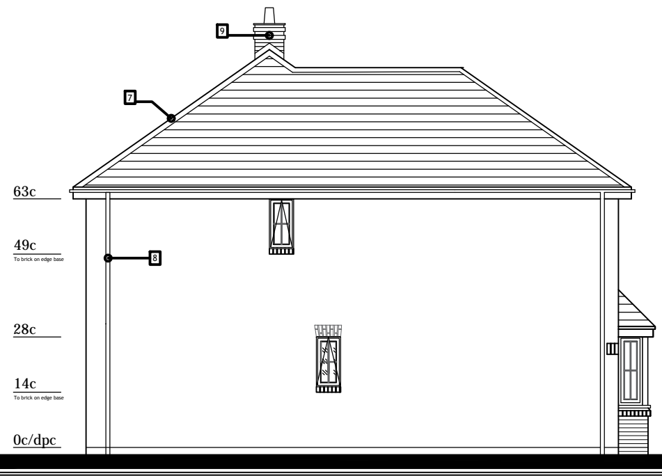
Side Elevation 1:100
