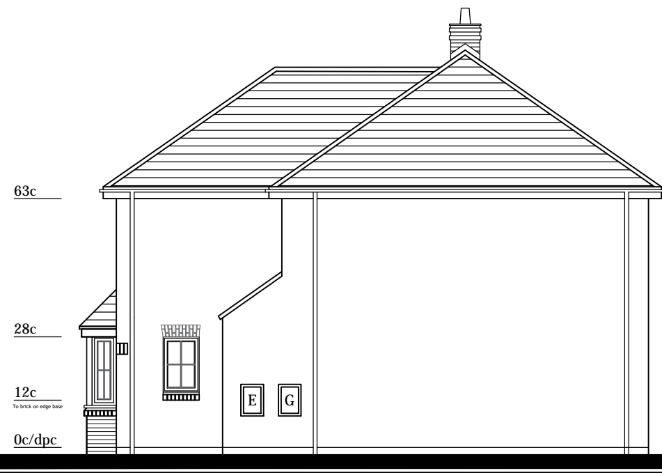
Side Elevation 1:100
