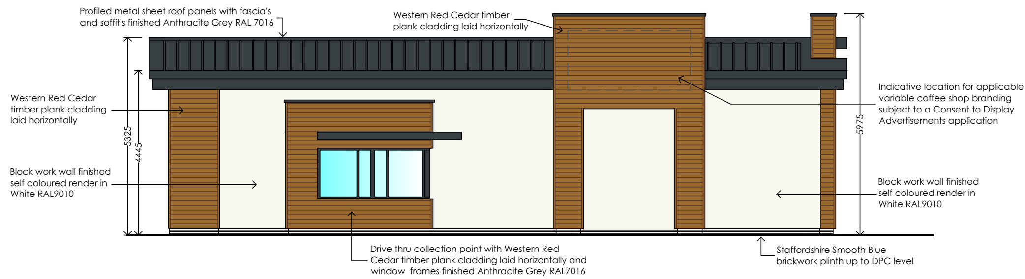
ELEVATION TO DRIVE THRU LANE AND COLLECTION POINT FACING SCHOOL ROAD
