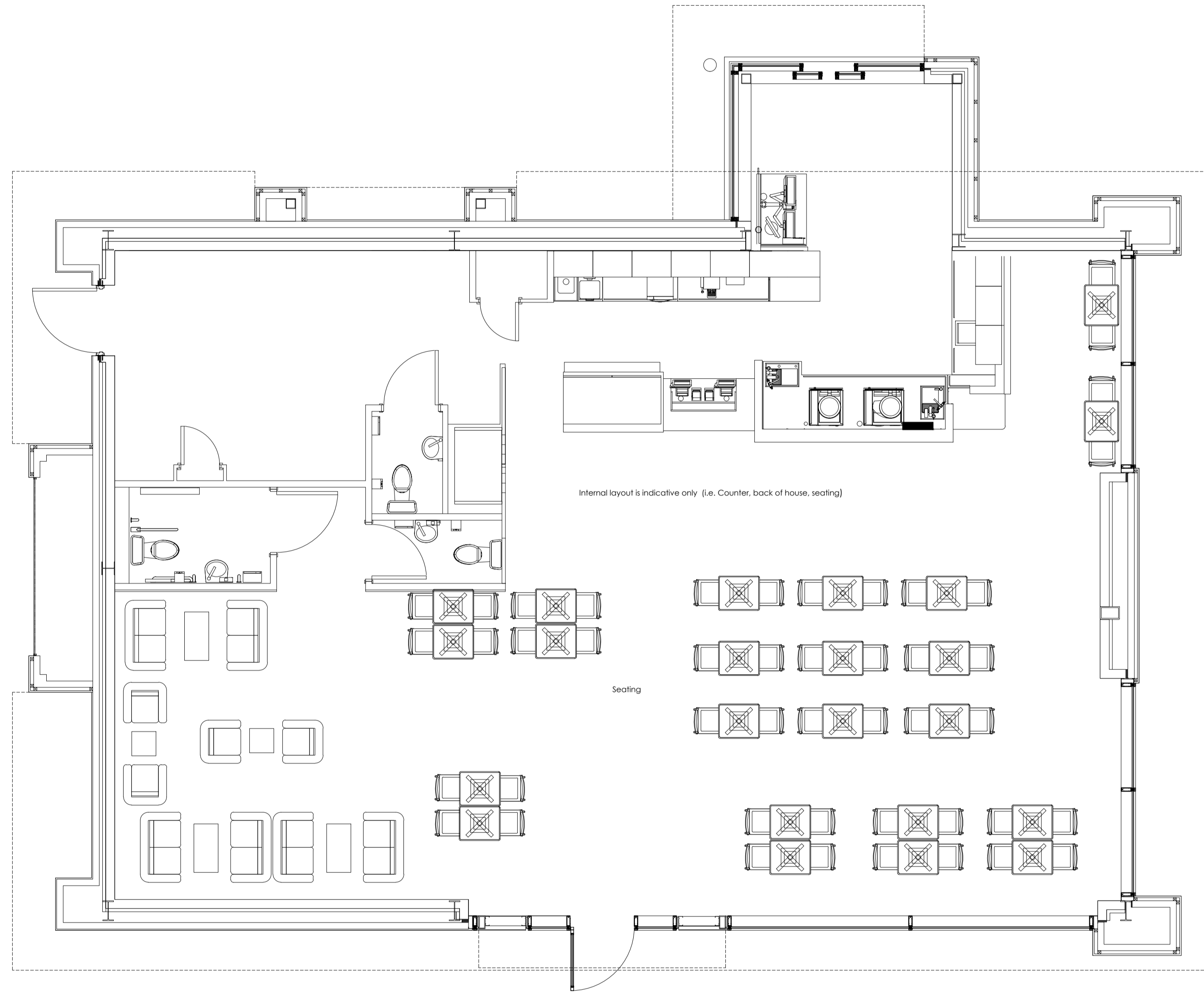
Building Plan Scale 1:50
